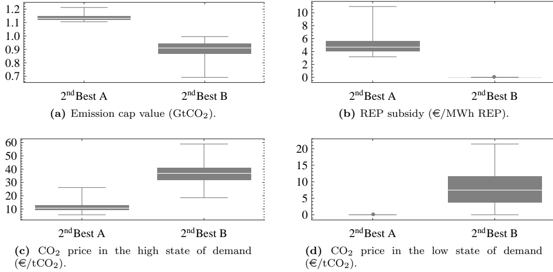
Figure 6: Box Whisker plot of various instrument levels and CO 2 price in all simulations with a nil CO 2 price in the low state of demand (2 nd Best A) and a strictly positive CO 2 price in the low state of demand (2 nd Best B).
