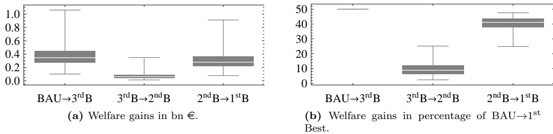
Figure 3: Box Whisker Plots of expected welfare gains from one scenario to another (BAU to 3 rd Best, 3 rd Best to 2 nd Best A, 2 nd Best A to 1 st Best) in all scenarios where the CO 2 price is nil in the low demand state of the world.
