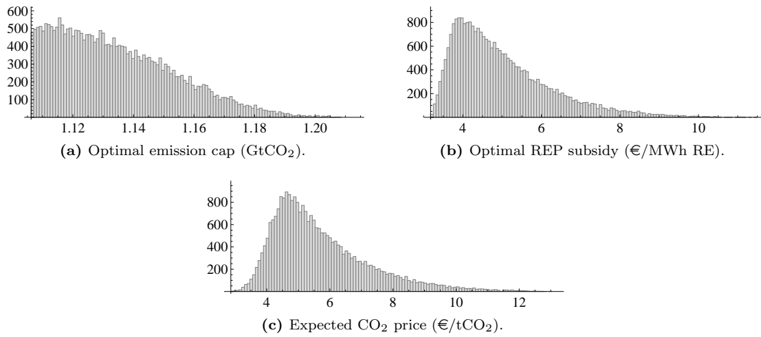
Figure 2: Histogram of the number of simulations per optimal policy instrument values and expected CO 2 price for all simulations with a nil carbon price in the low demand state of the world.
