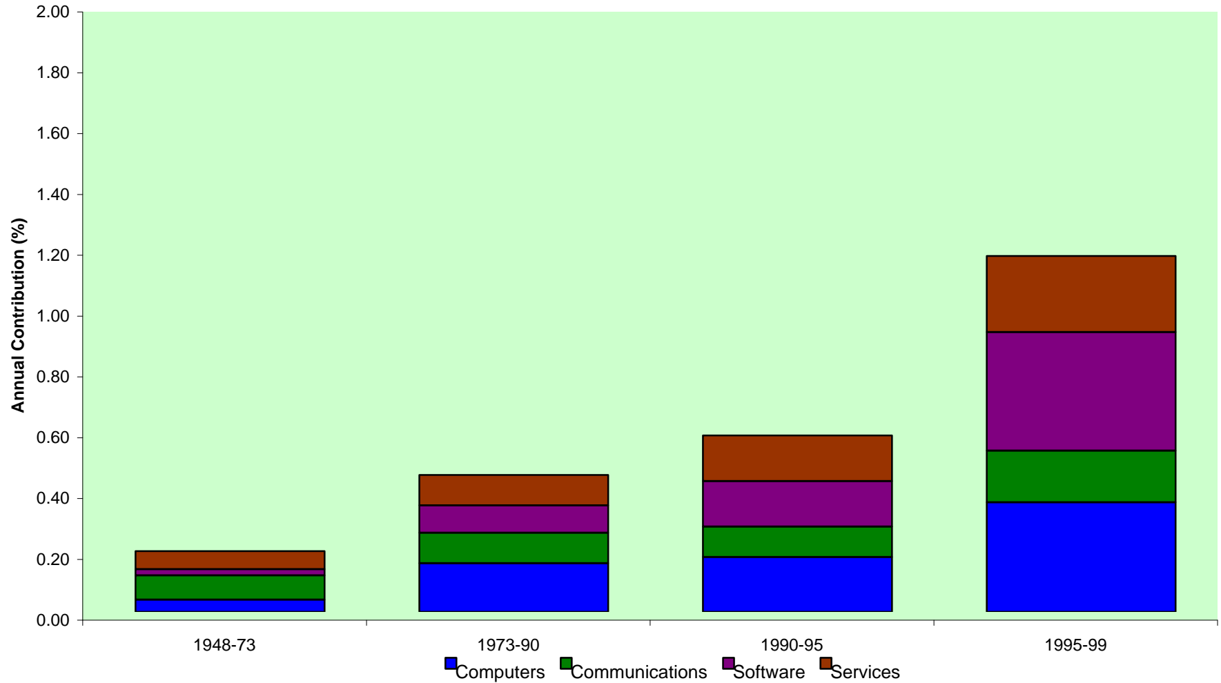
Chart 7: Output Contribution of Information Technology by Type
