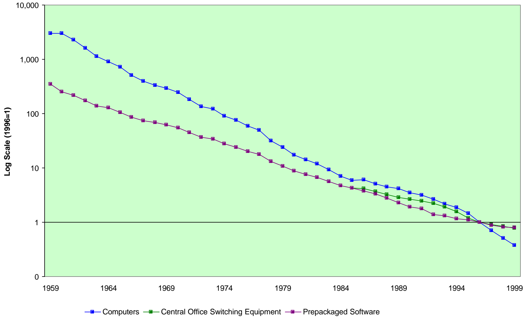
Chart 3: Relative Prices of Computers, Communications, and Software, 1959-1999
