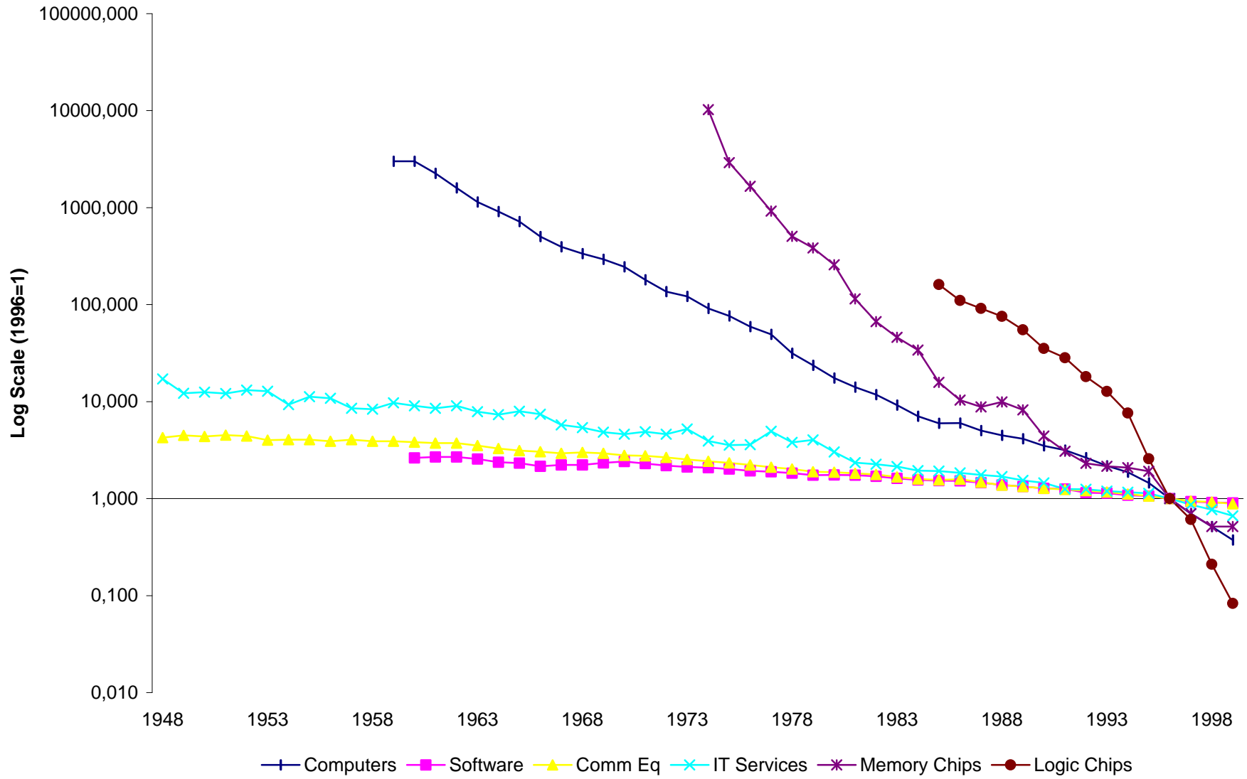
Chart 3b: IT Deflators, 1948-99
