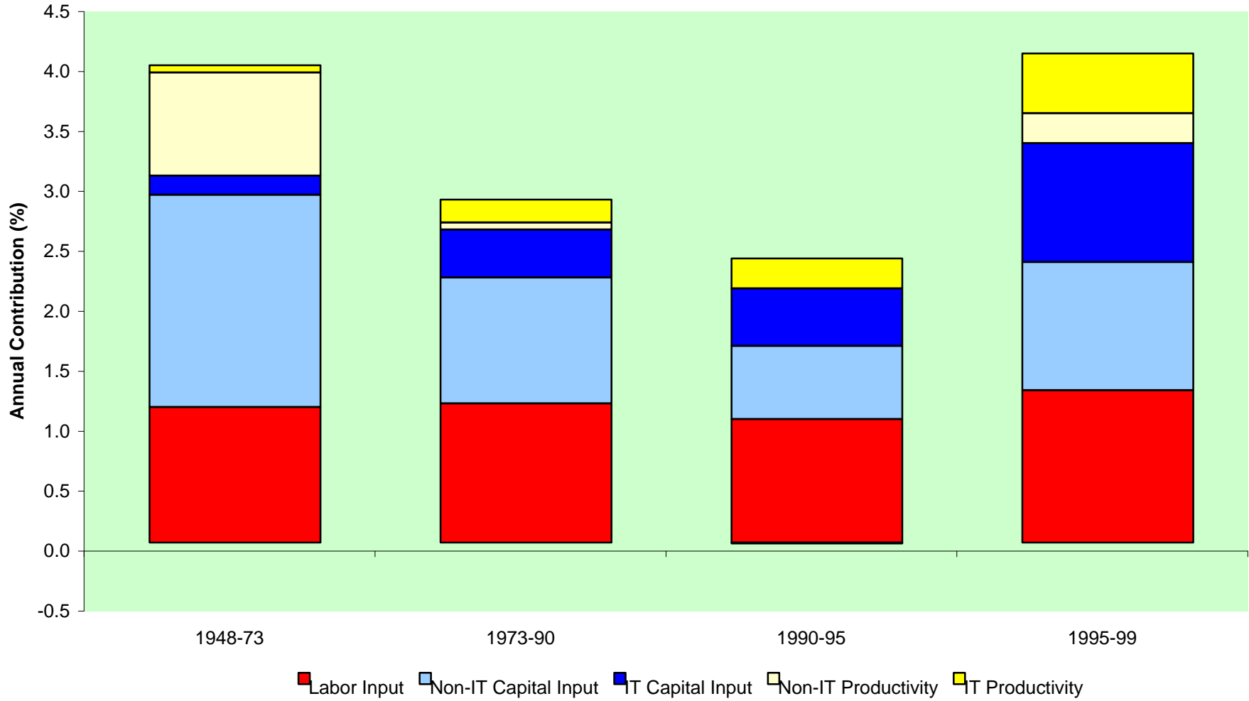
Chart 11: Sources of Gross Domestic Product Growth
