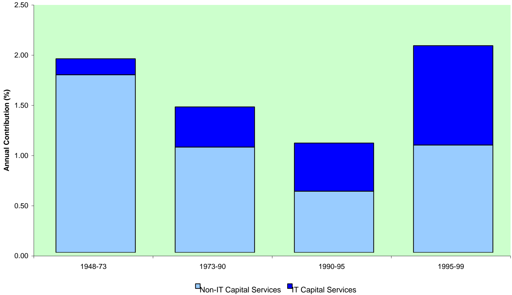
Chart 8: Capital Input Contribution of Information Technology
