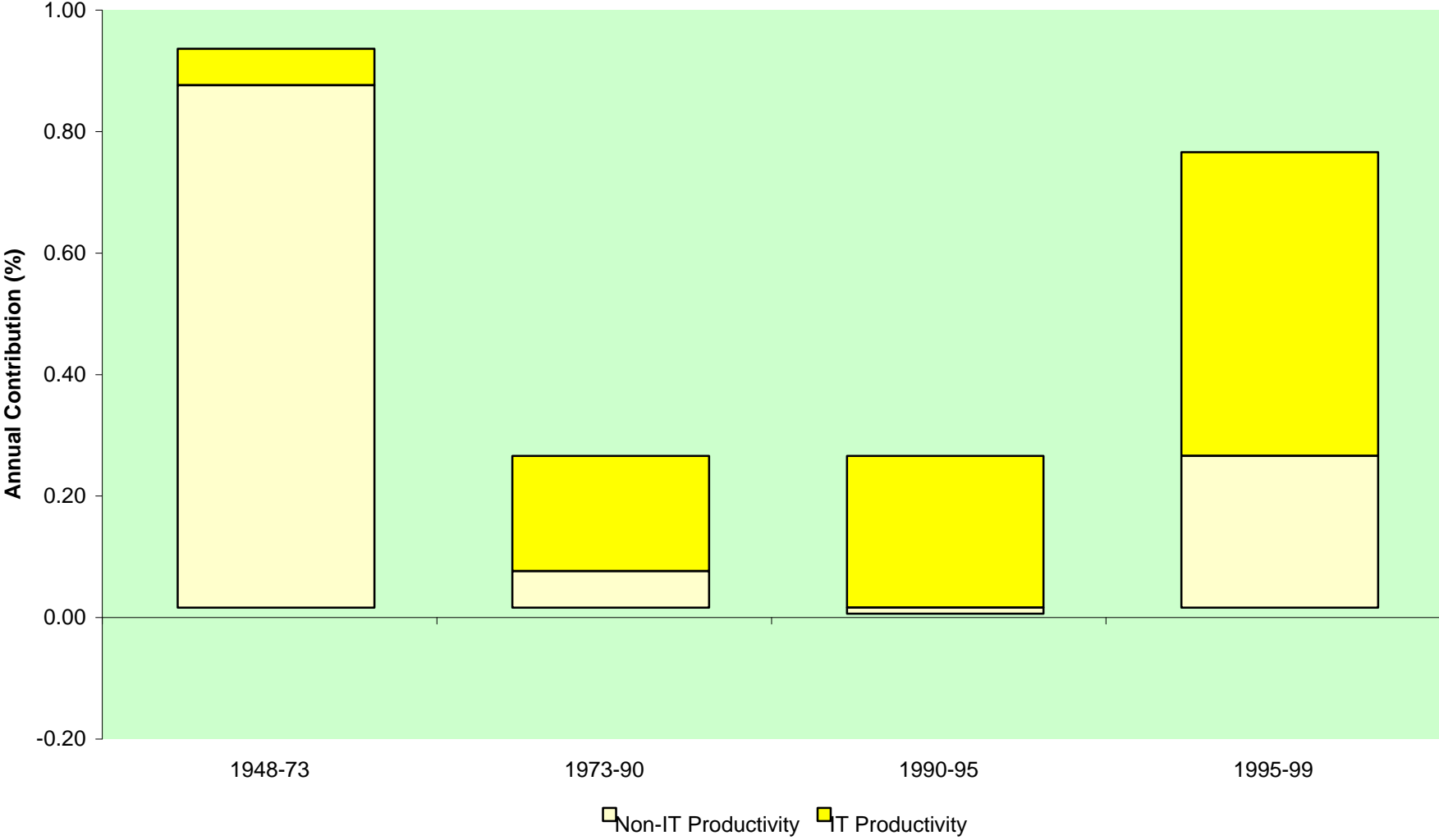
Chart 10: Contributions of Information Technology to Total Factor Productivity Growth
