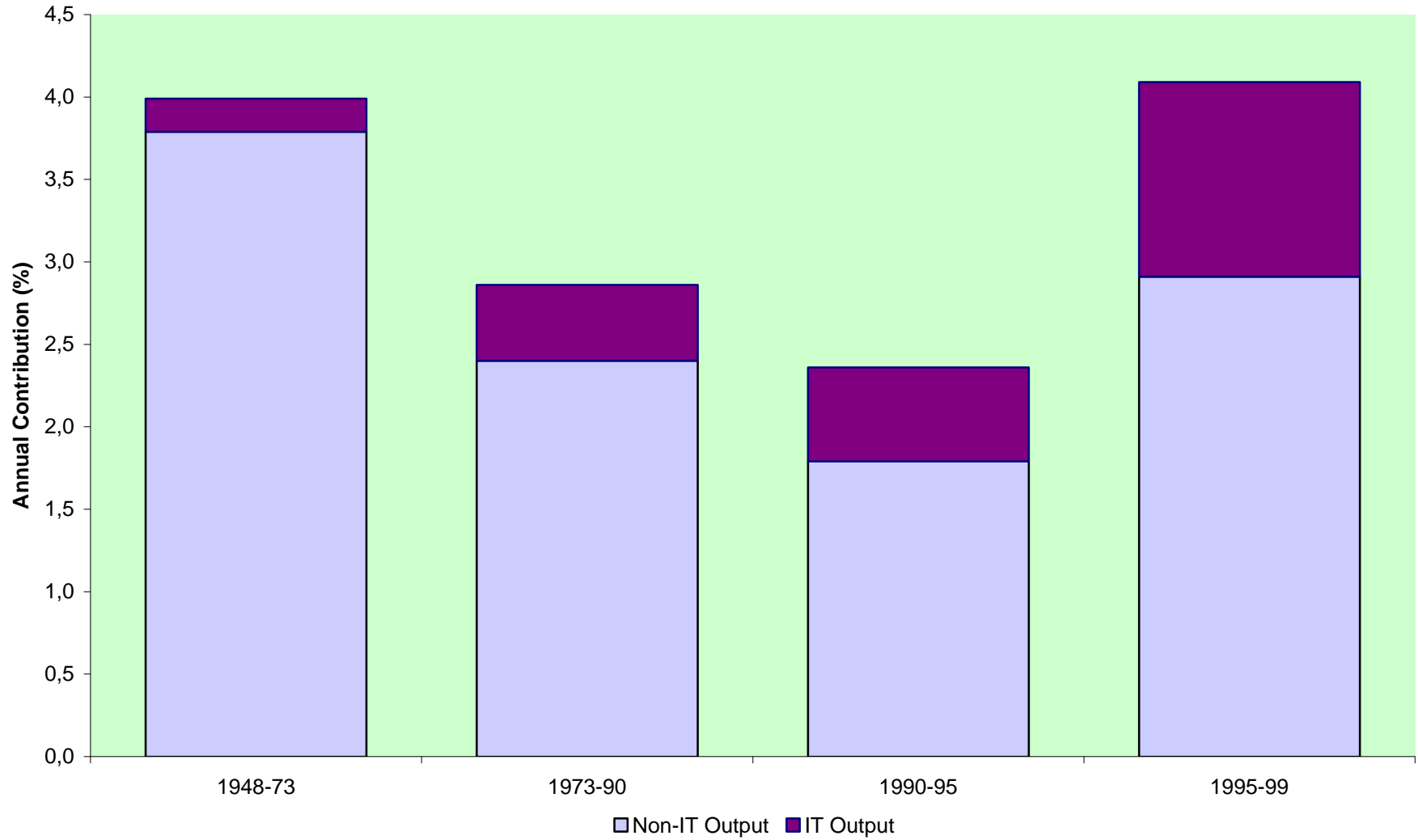
Chart 7: Output Contribution of IT, 1948-99
