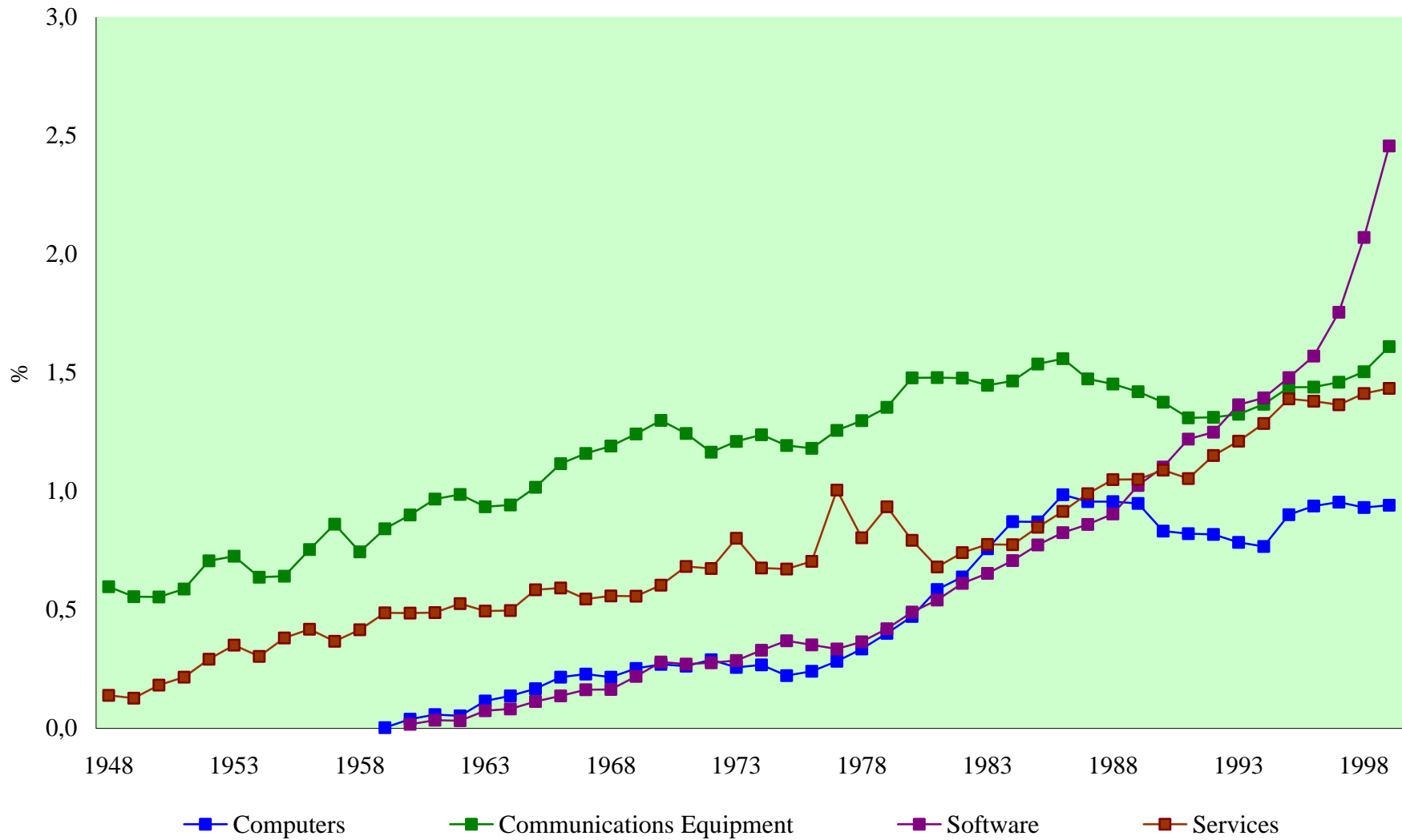
Chart 5: Output Shares of Information Technology by Type, 1948-99
