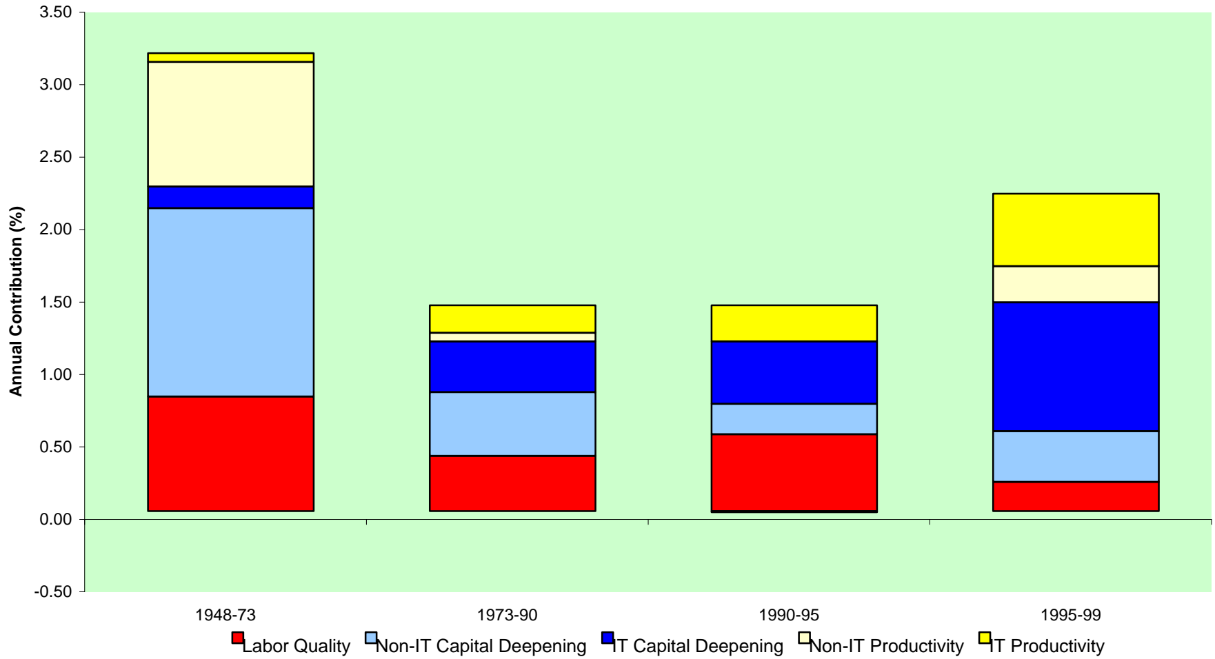
Chart 12: Sources of Average Labor Productivity Growth
