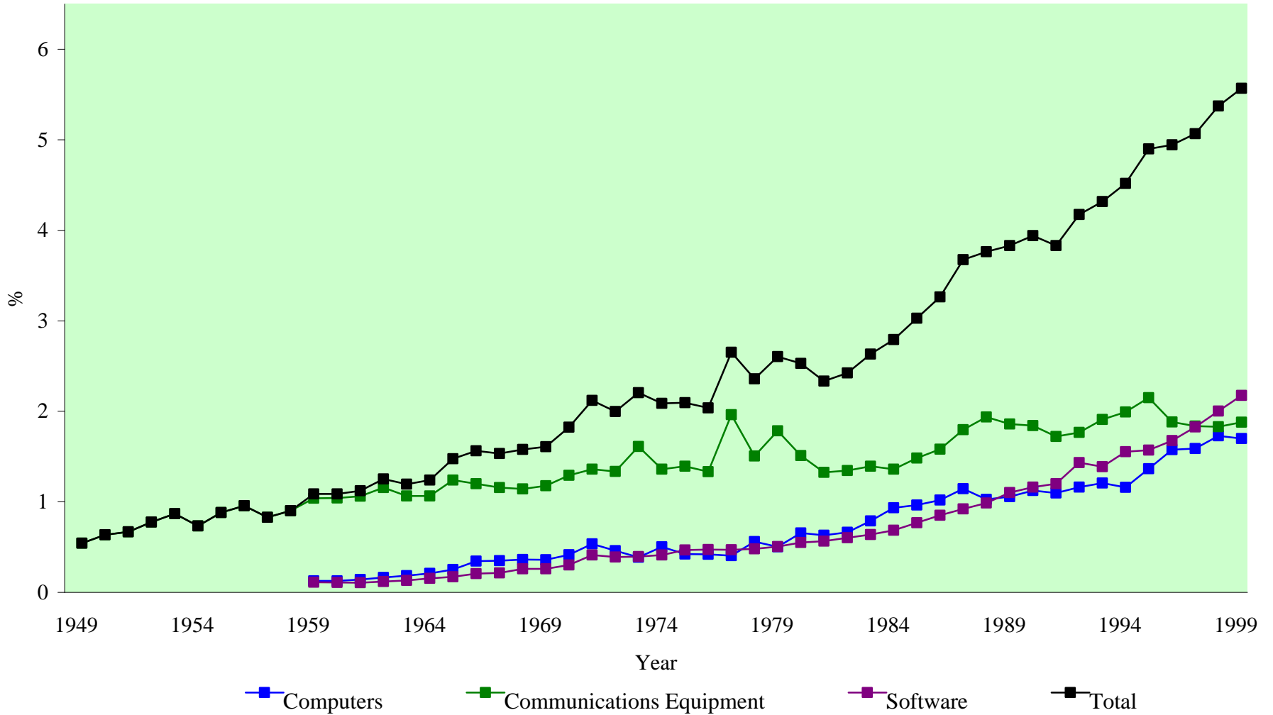
Chart 5: Input Shares of Information Technology by Type, 1948-99
