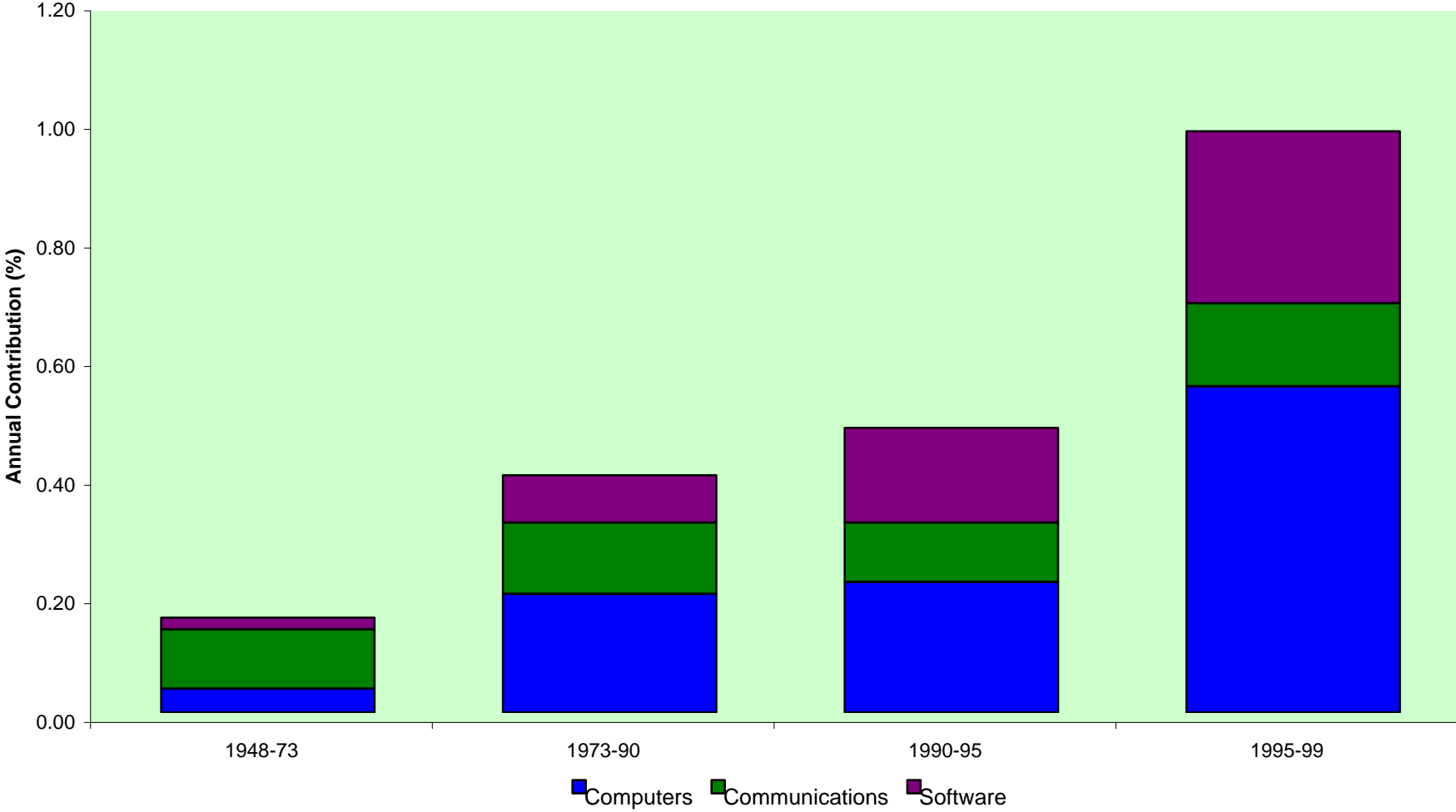
Chart 9: Capital Input Contribution of Information Technology by Type
