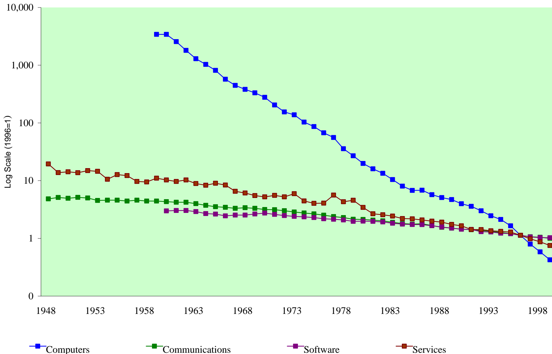
Chart 2: Relative Prices of Computers, Communications, Software, and Services, 1948-99
