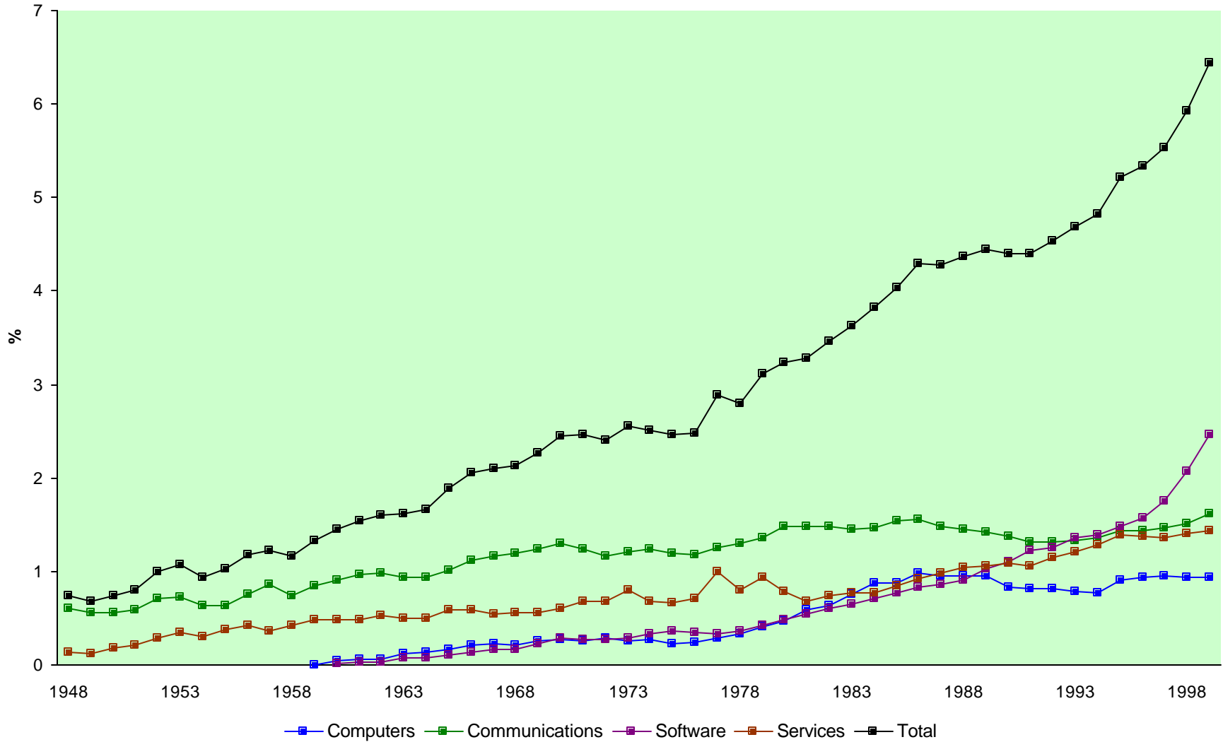
Chart 4: Output Shares of Information Technology by Type, 1948-99
