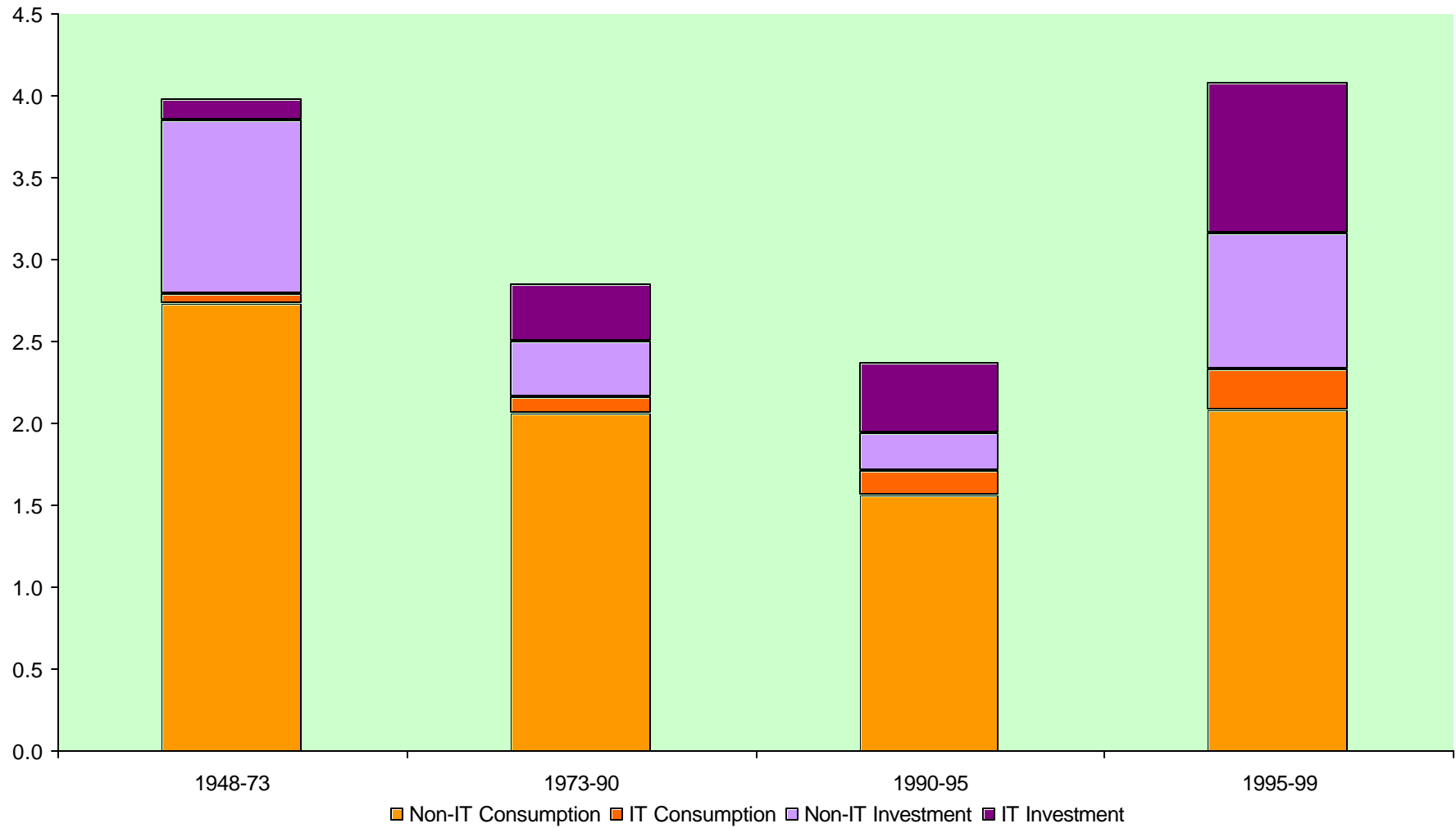
Chart 6: Output Contribution of Information Technology
