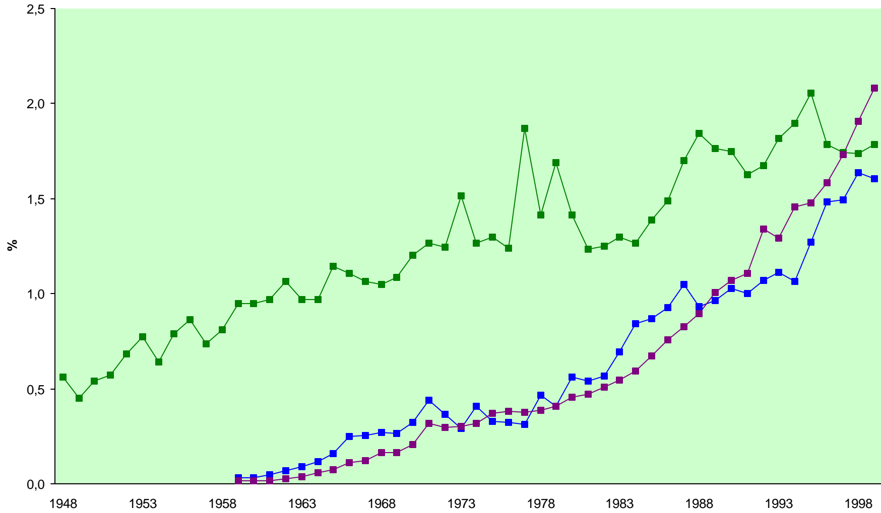
Chart 6: Input Shares of Information Technology by Type, 1948-99
