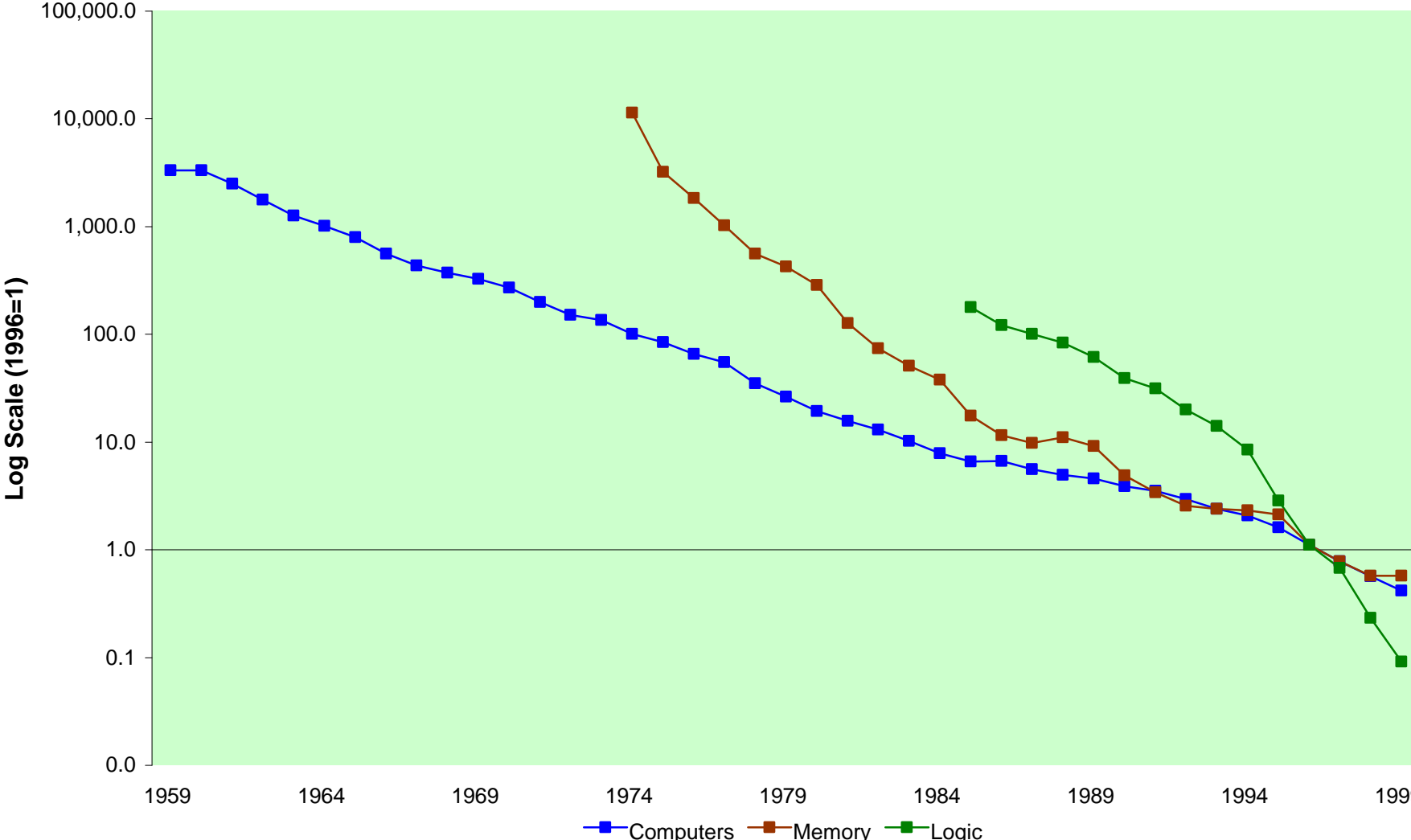
Chart 1: Relative Prices of Computers and Semiconductors, 1959-1999
