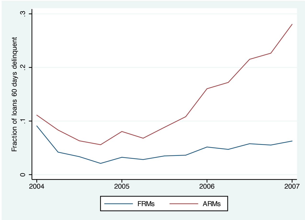
Figure 4: Delinquency rates for ARMs and FRMs issued in 2003
