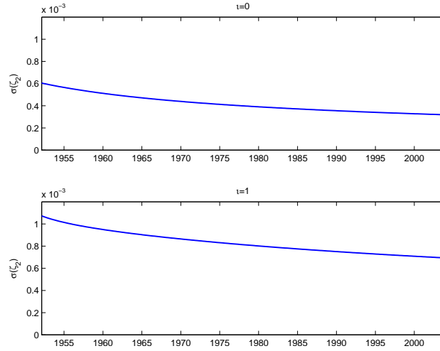
Figure 6: Standard deviation of \zeta(0) (top panel) and of \zeta_2(1) (bottom panel).
