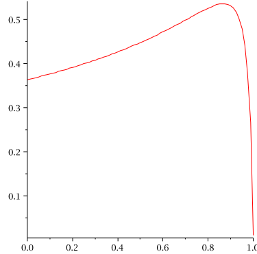
Figure 2: Network externalities function for weak protection; \lambda = 10 , q^+ = 0.5 , p^+ = 0.01 and q = 0.1
