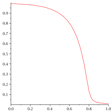
Figure 1: Network externalities function for strong protection; \lambda = 10 , q^+ = 0.5 , p^+ = 0.01
