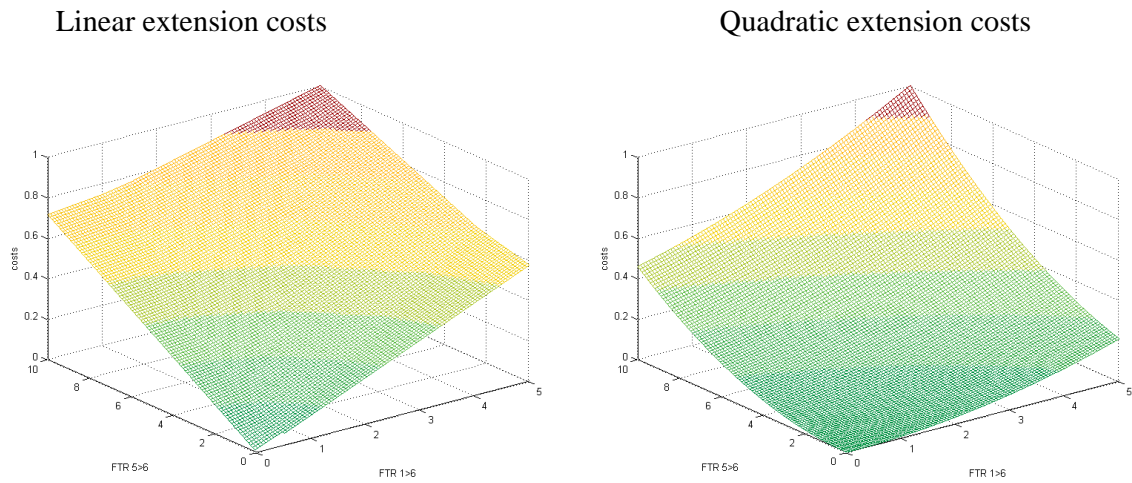
Figure 11: Global cost function, six-node network, fixed reactances
