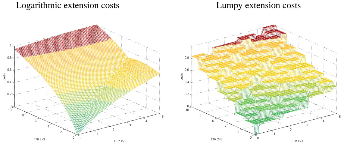
Figure 4: Global cost function, three-node network, fixed reactances
