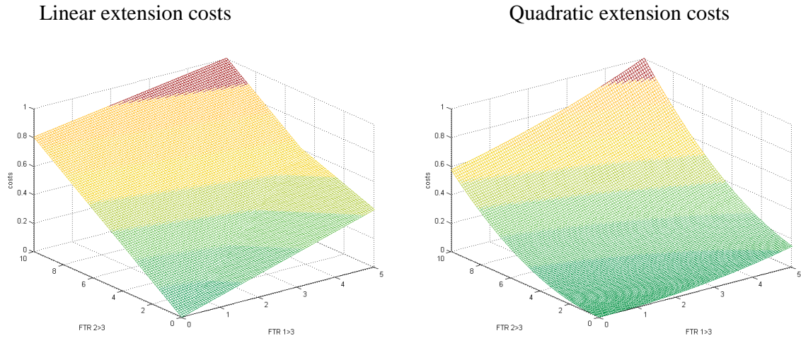
Figure 10: Global cost function, three-node network, fixed reactances
