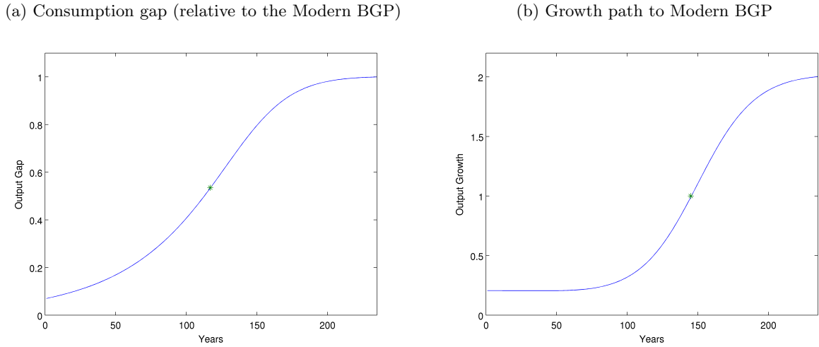
Figure 4: Slow transitional dynamics.
