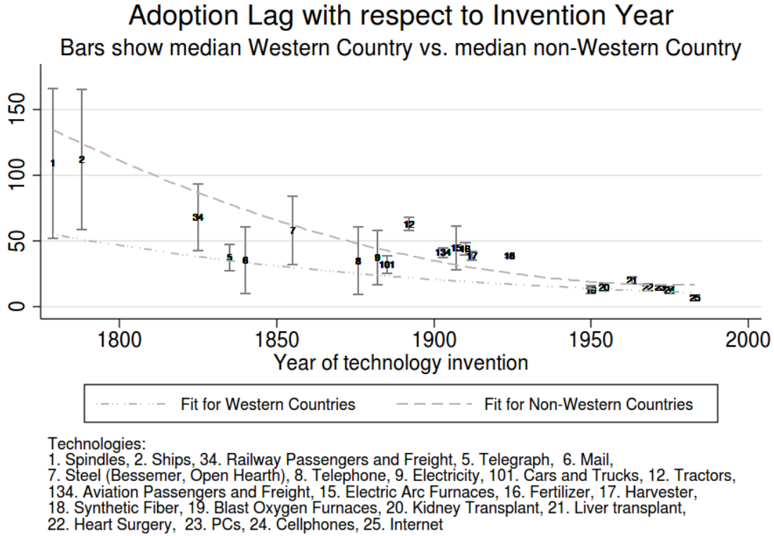
Figure 2: Convergence of Adoption Lags
