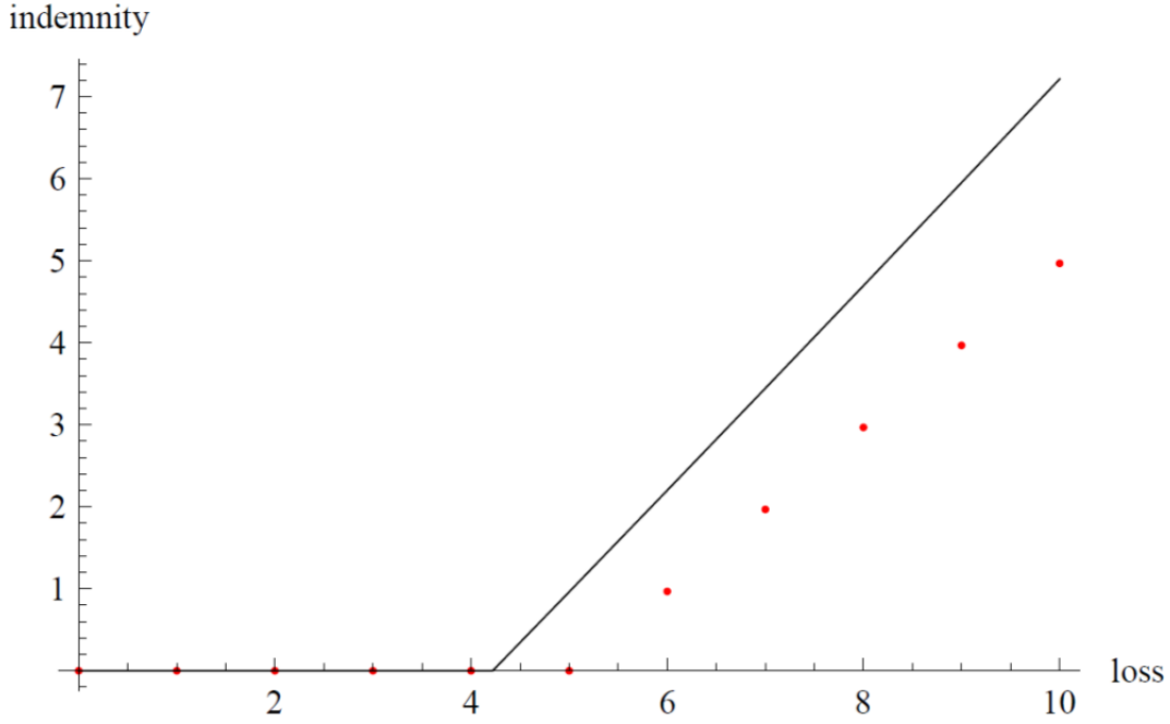
Figure 3: Optimal contract under a two-state ambiguity structure. The support of loss is \{0,1,\dots,10\} . There are two equally likely cdfs, respectively with probabilities (11/66,10/66,\dots,1/66) and (1/66,2/66,\dots,11/66) . We also assume u(c) = \sqrt{c}/2 , w_0 = 11 and \tau = 0.11 . The dots correspond to the optimal insurance schedule under ambiguity neutrality, whereas the plain curve is the optimal contract if \phi(u) = -e^{-u} .
